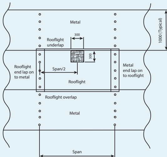
Diagram 4. Single-span rooflight WORST CASE IMPACT POSITION
