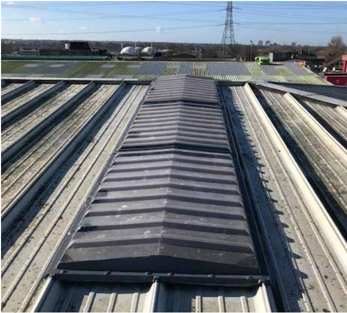
Old rooflights before refurbishment
